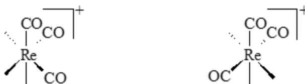
Figure 1. Complex compounds containing a [\text{Re}(\text{CO})_3]^+ core, with facies geometry (left) and meridional geometry (right). To increase the clarity of the figure, the remaining ligands have been omitted.
